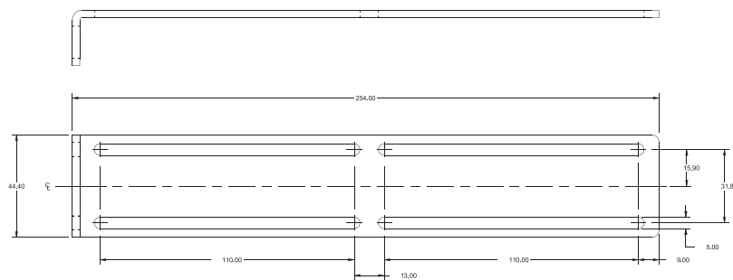
Adjustable PDU bracket for button mounting
