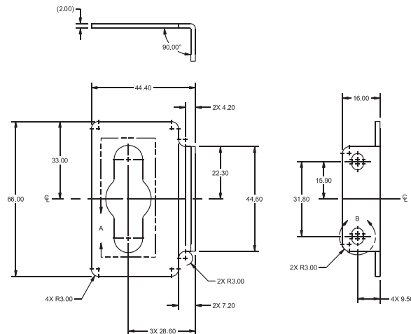
Adjustable PDU bracket for button mounting
