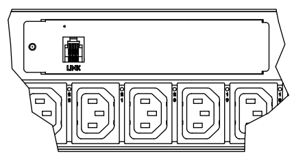
DETAIL A LINK OPTION SCALE 1 / 3
