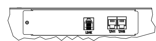
DETAIL A SCALE 0.36 : 1
